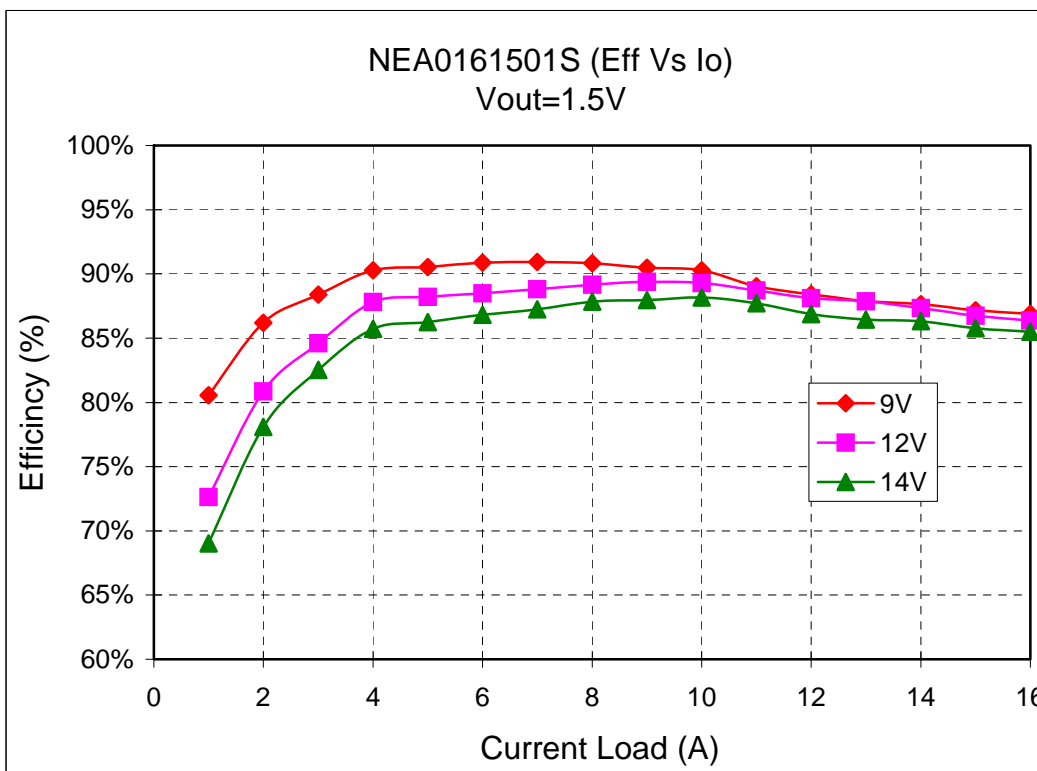
Fig 22. SMT Efficiency Curves for Vout=1.5V (25C)
